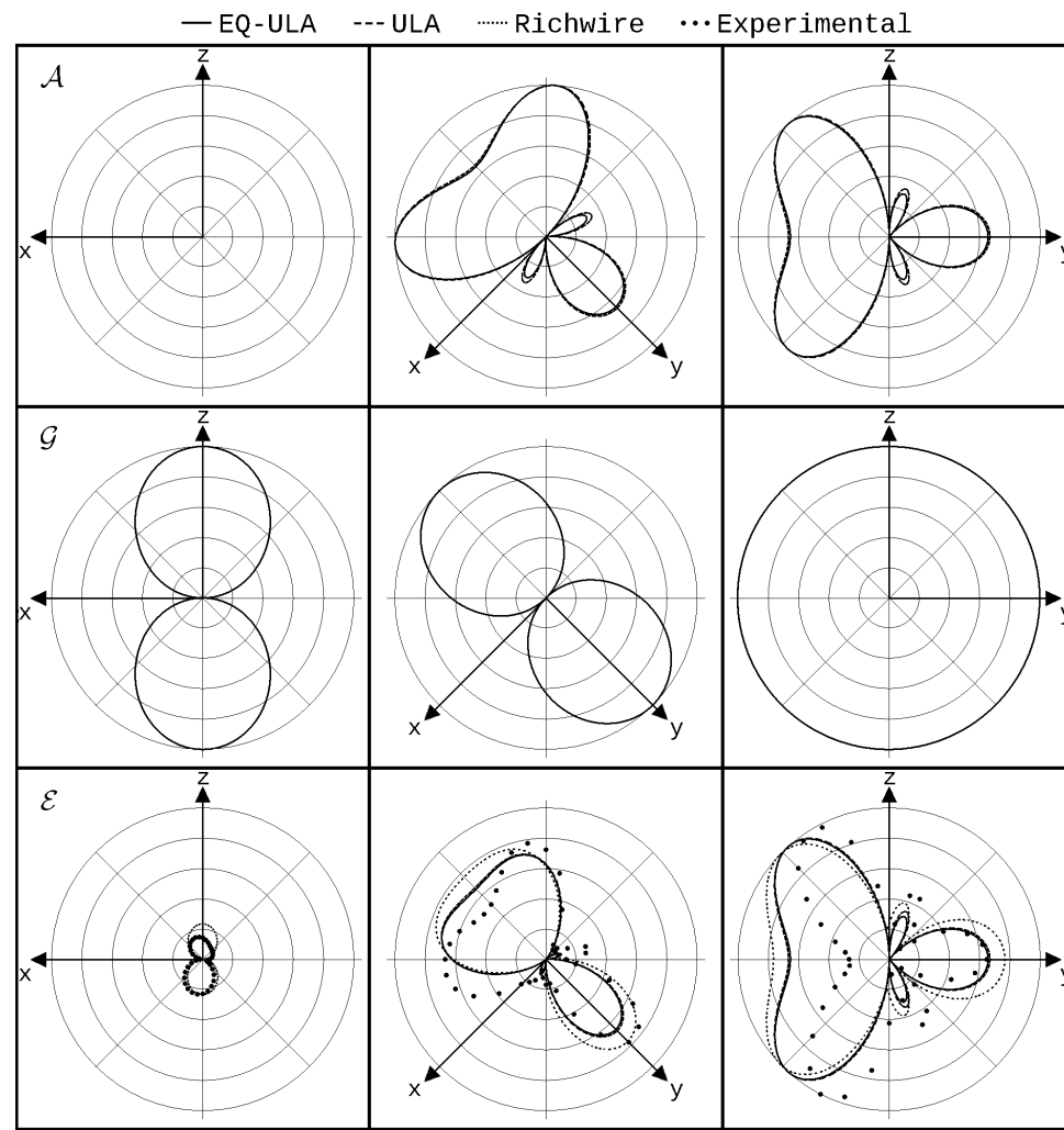
Fig. 23: Normalized 2D radiation patterns \mathcal{A}, \mathcal{G}, \mathcal{E}
