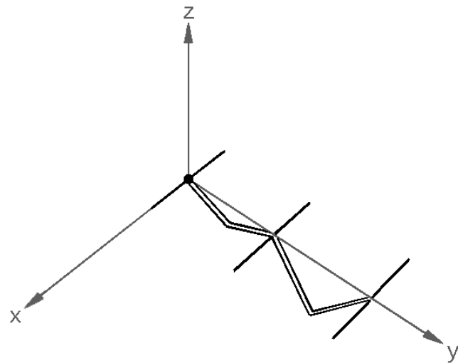
Fig. 19: The simulation model
