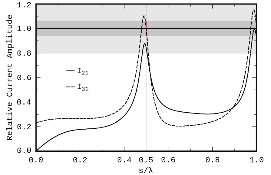
Fig. 9: Amplitude of current ratios for s = d = \ell
