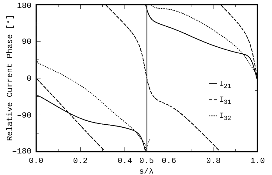
Fig. 10: Phase difference of current ratios for s = d = \ell
