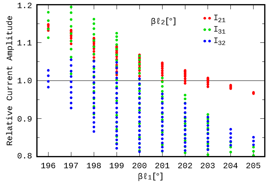
Fig. 16: Amplitude of current ratios for possible \beta_{l2} values
