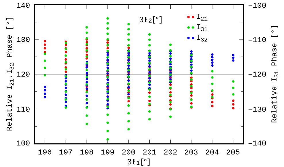
Fig. 17: Phase of current ratios for possible \beta_{l2} values
