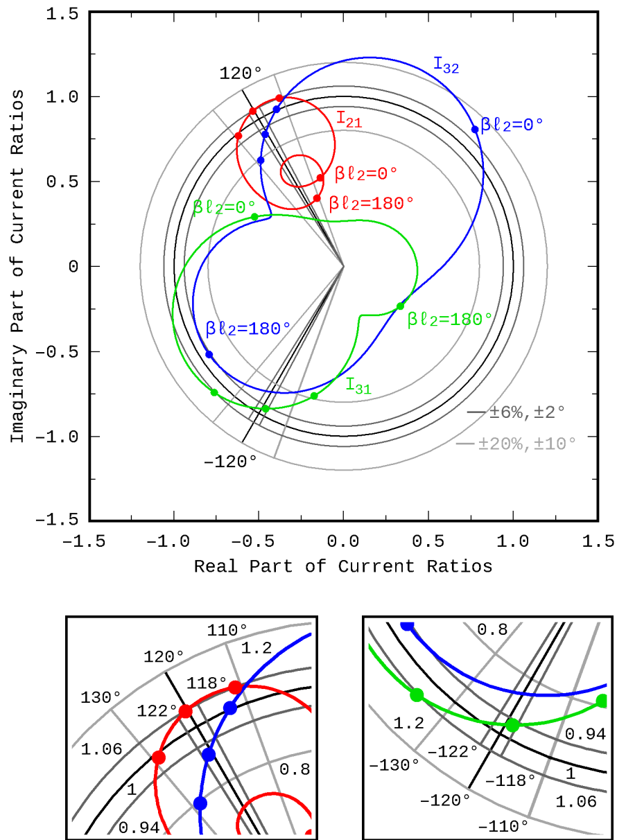
Fig. 18: Currents ratios versus \beta l_2 with \beta l_1 = 200^\circ
