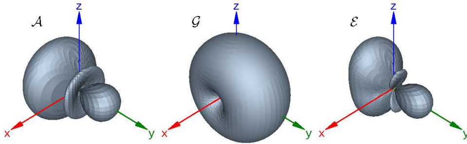
Fig. 24: Multiplication Principle: 3D patterns in dB [5]
