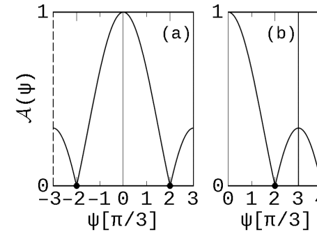
Fig. 12: ULA Array Factor A
